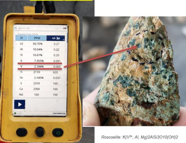
Previsto hand sample – Roscoelite
